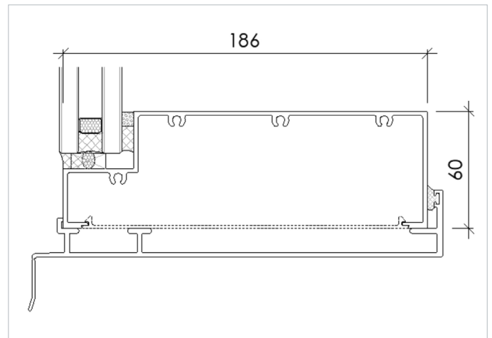
Subsill
