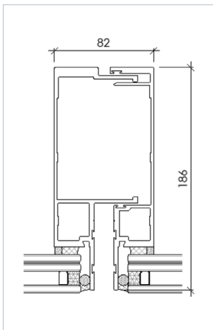
Standard mullion
